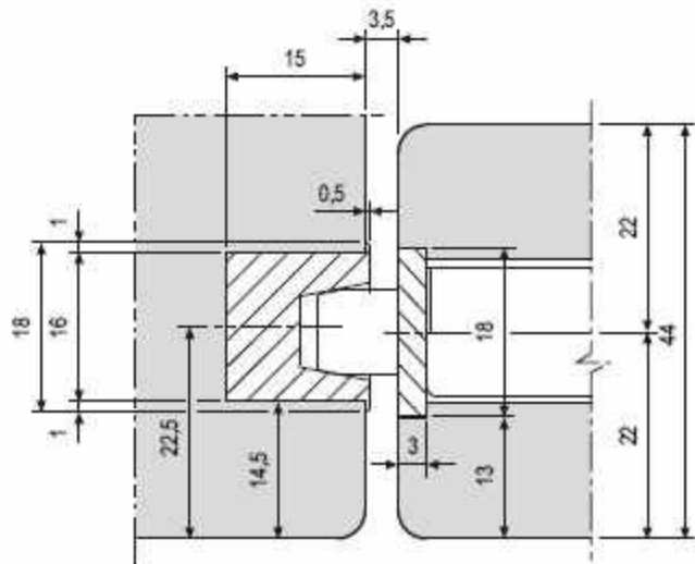
Example of swinging application
