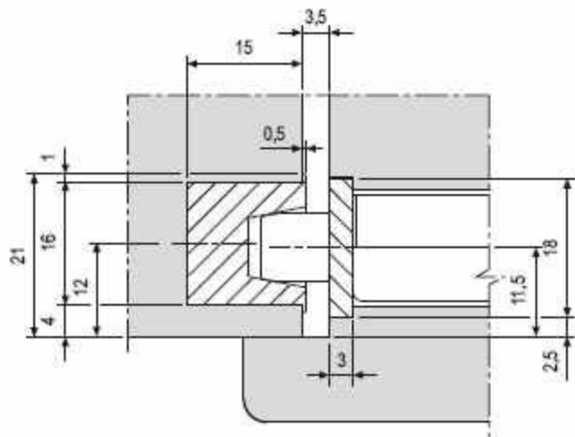
Example of swinging application
